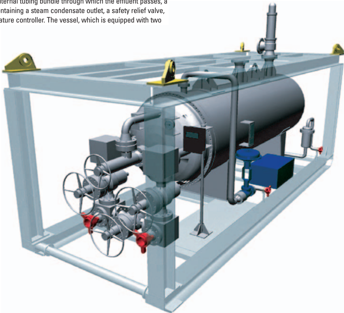
Steam-heat exchanger.
