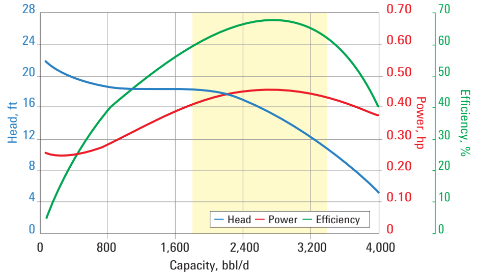
A2700N pump curve for 60 Hz with sg = 1.
