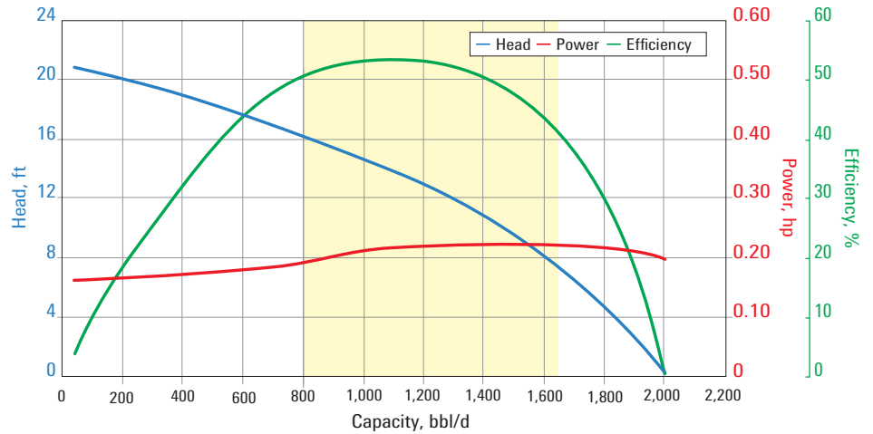
AN1200 pump curve for 60 Hz with sg = 1 .
