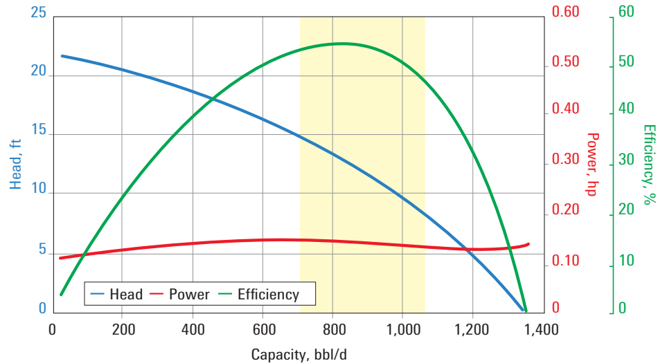
AN900 pump curve for 60 Hz with sg = 1 .
