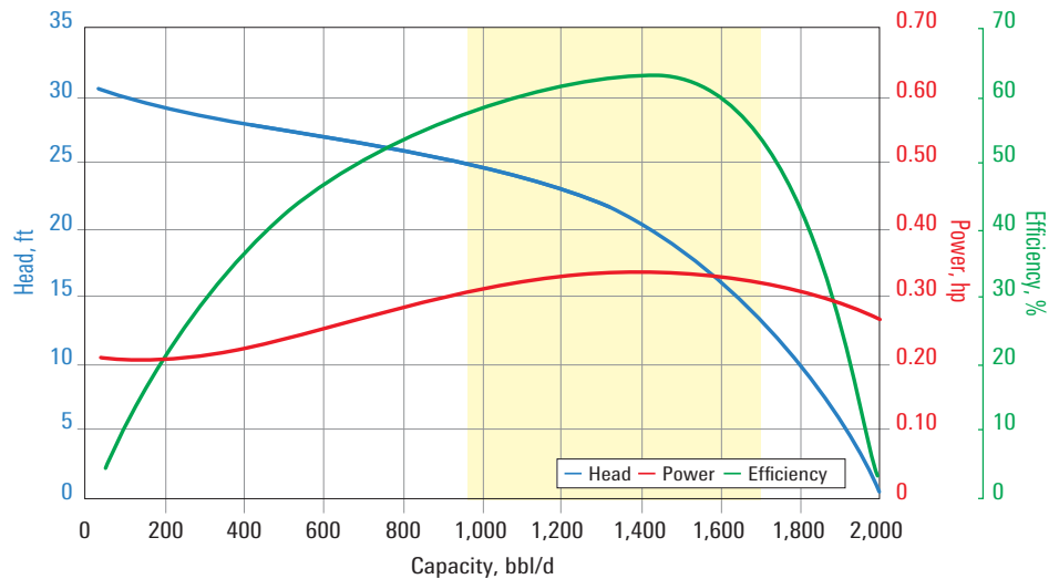
D1400N pump curve for 60 Hz with sg = 1.
