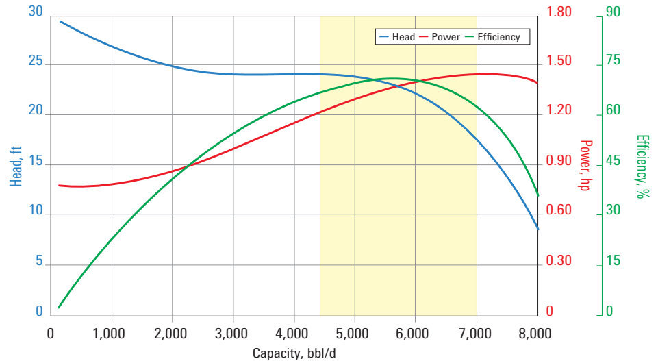
D5800N pump curve for 60 Hz with sg = 1 .
