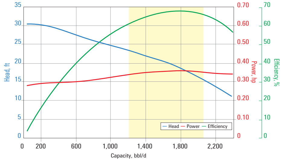
DN1750 pump curve for 60 Hz with sg = 1.
