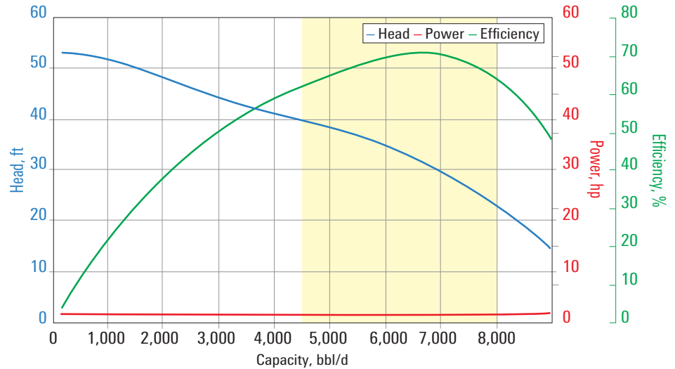
G6200N pump curve for 60 Hz with sg = 1 .
