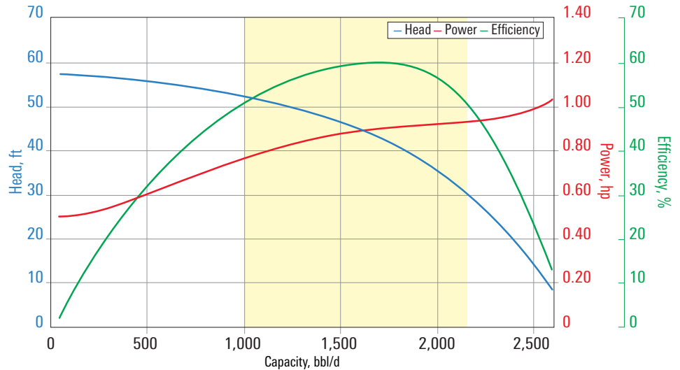
GN1600 pump curve for 60 Hz with sg = 1 .
