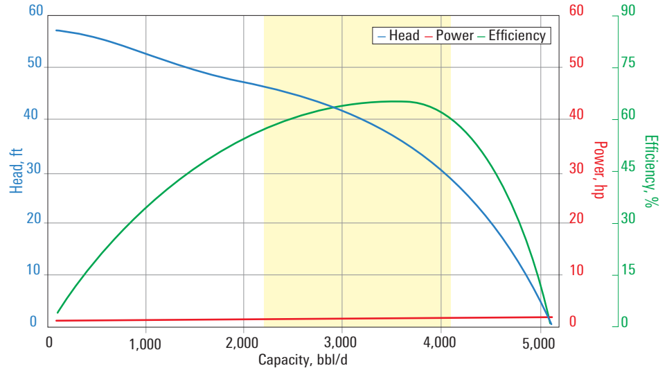
GN3200 pump curve for 60 Hz with sg = 1 .
