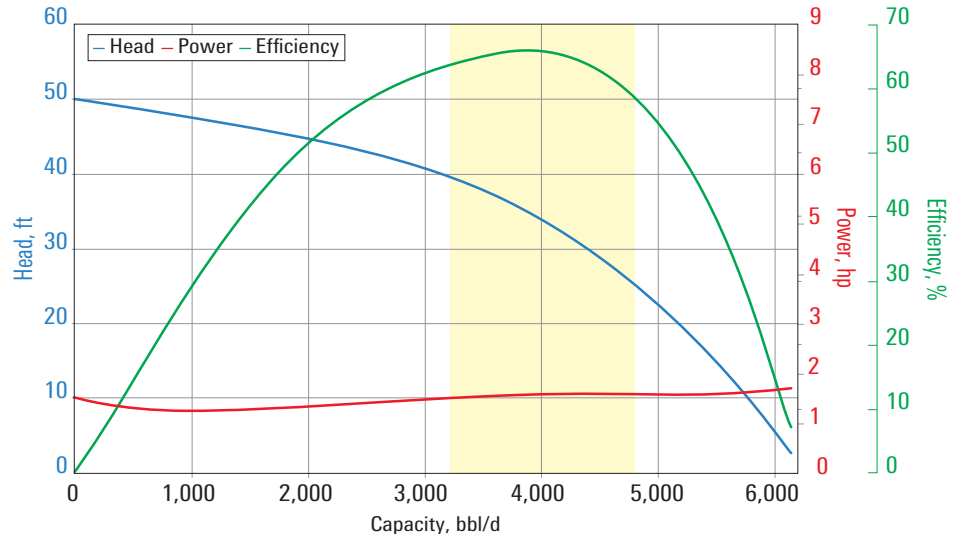
GN4000 pump curve for 60 Hz with sg = 1 .
