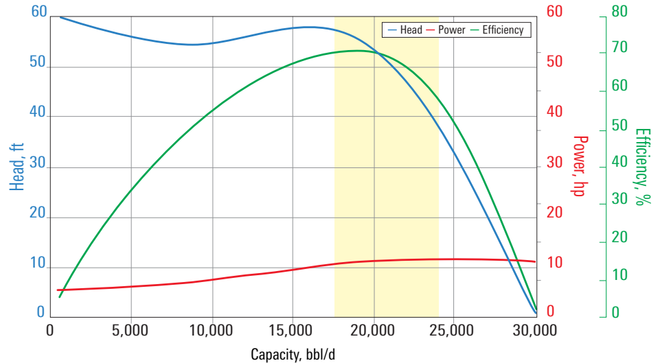
H21500N pump curve for 60 Hz with sg = 1 .
