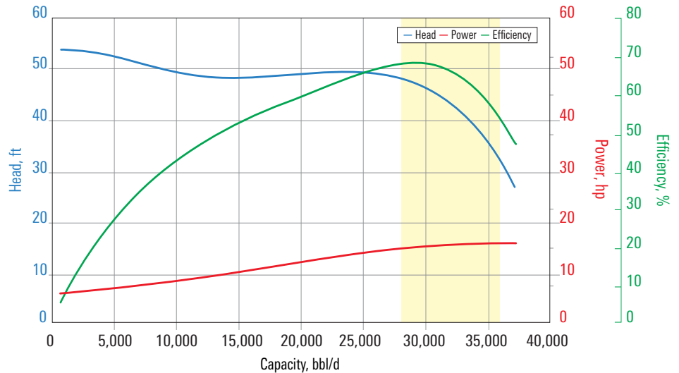
H28000N pump curve for 60 Hz with sg = 1 .
