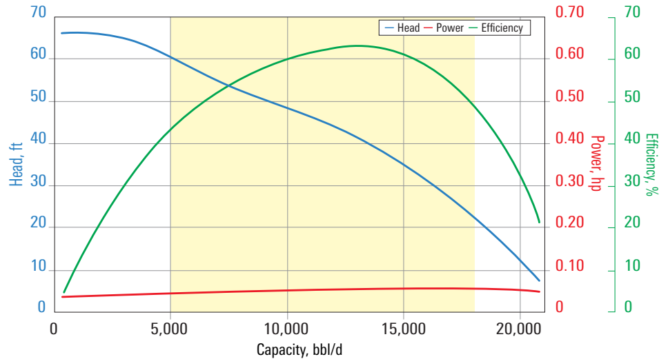
HN13500 pump curve for 60 Hz with sg = 1 .
