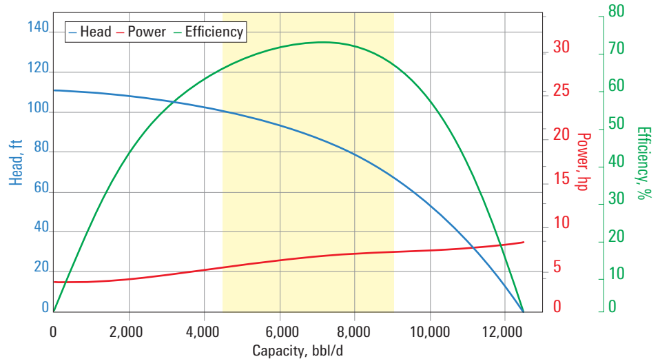
J7000N pump curve for 60 Hz with sg = 1 .
