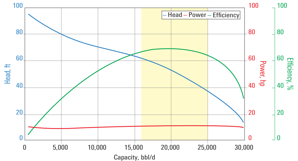
JN21000 pump curve for 60 Hz with sg = 1 .
