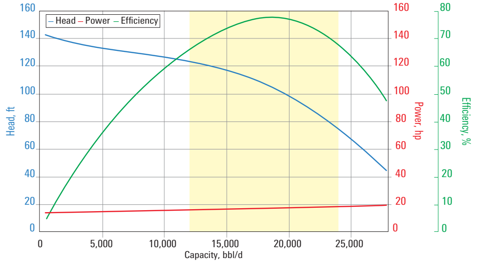
M520A pump curve for 60 Hz with sg = 1 .
