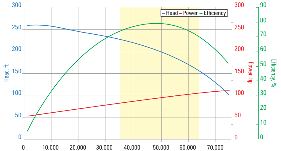
N1400NA pump curve for 60 Hz with sg = 1 .
