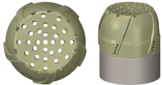
20-in × 22-in XCDR 513 reamer.
