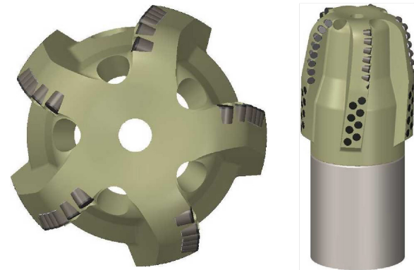
5½-in × 7⅞-in XCDR 513 reamer.
