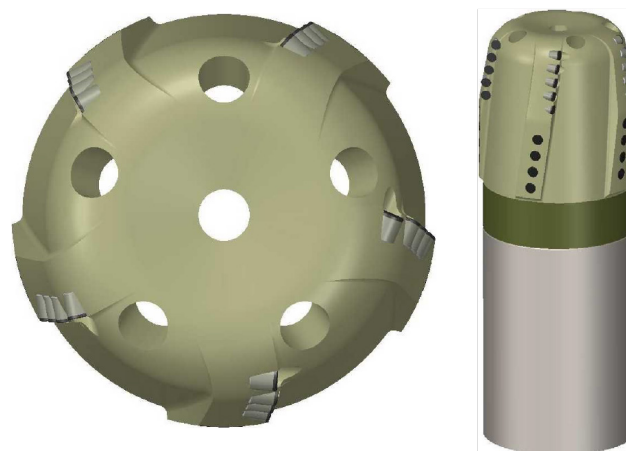
7 5 / 8 -in × 8 1 / 4 -in XCDR 513 reamer.
