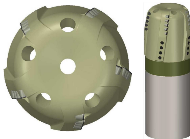
7-in × 8¼-in XCDR 513 reamer.
