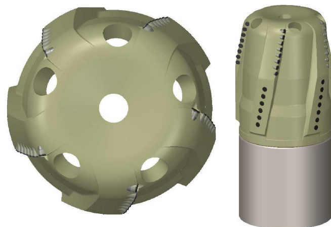
9 5 / 8 -in × 11 1 / 2 -in XCDR 513 reamer.
