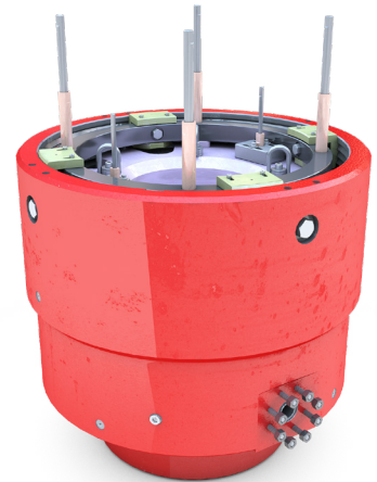
Assembly and disassembly tool for 18 3 / 4 DL annular BOP.
