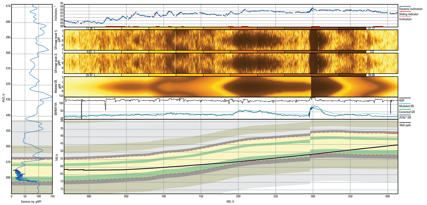
GR imaging from the TelePacer platform guides steering decisions, provides dips, reveals faults, and helps improve in-zone percentage.
