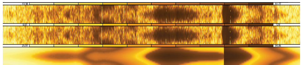
Real-time gamma ray imaging confirms geological model while drilling.
