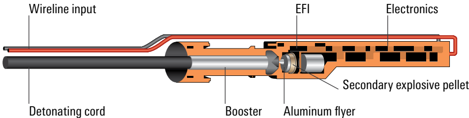
Secure2 electronic detonator.
