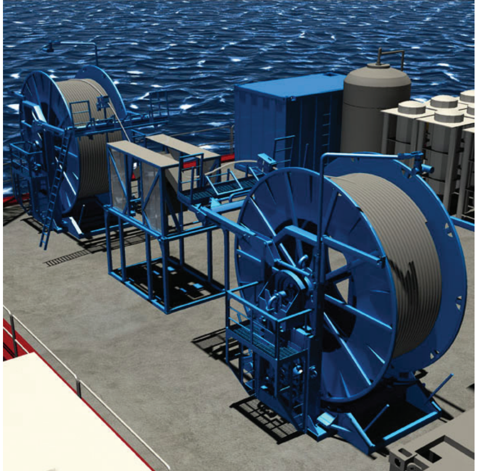
The ReelCONNECT system extends CT applications to deeper wells.
